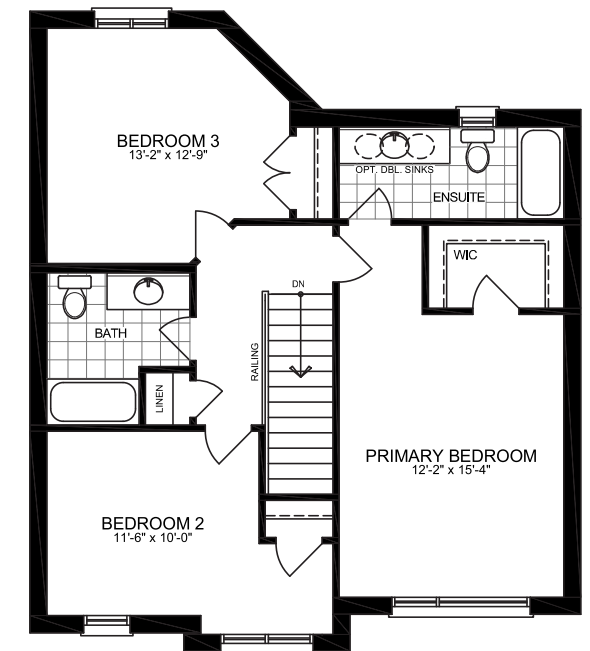
ELEVATION 'B' - SECOND FLOOR PLAN - 912 SQ. FT.
