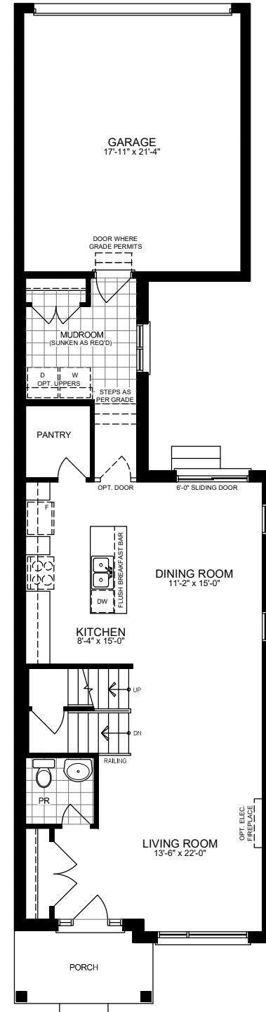
ELEVATION 'B' - MAIN FLOOR PLAN - 998 SQ. FT.
