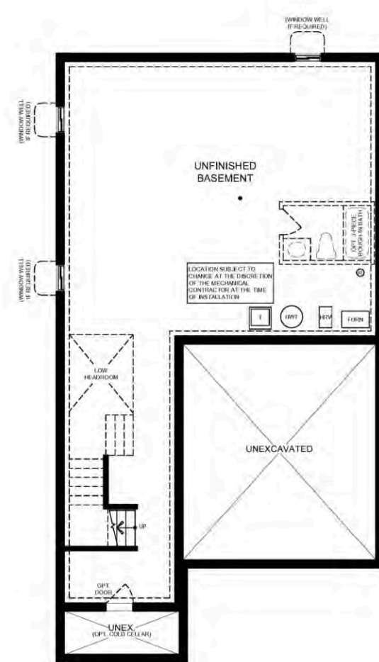
ELEVATION 'B' - BASEMENT PLAN
