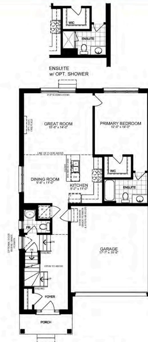
ELEVATION 'B' - MAIN FLOOR PLAN - 1070 SQ. FT.
