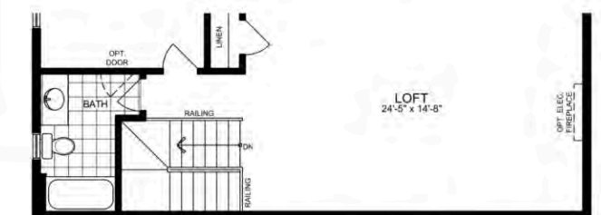
ELEVATION 'A' - SECOND FLOOR PLAN - 738 SQ. FT.
