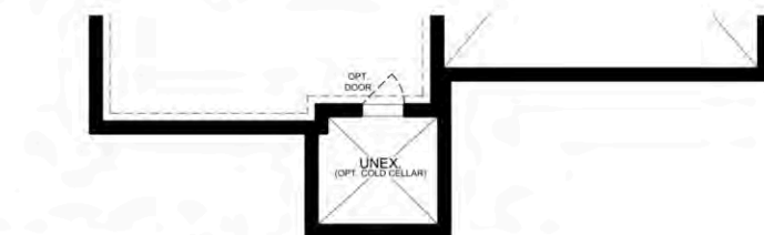
ELEVATION 'A' - OPT. FIN. BASEMENT PLAN - 794 SQ. FT.
