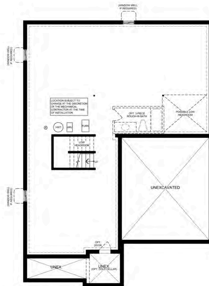
ELEVATION 'B' - BASEMENT PLAN
